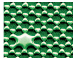
Ordered arrays of silicon pillars with controlled height and aspect ratio A Sinitski et al 2007 Nanotechnology 18 305307
