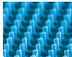
Fabrication of a dense array of tall nanostructures over a large sample area with sidewall profile and tip sharpness control C-H Choi and C-J Kim 2006 Nanotechnology 17 5326–5333
