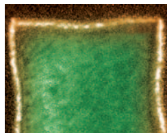
Morphology and oxide shell structure of iron nanoparticles grown by sputter-gas-aggregation C M Wang et al 2007 Nanotechnology 18 255603
